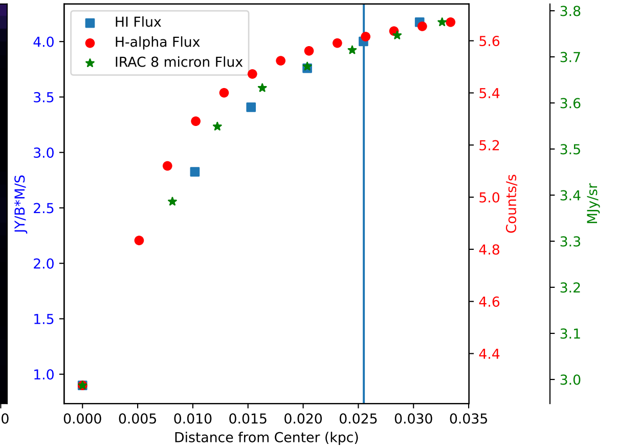
Flux of HI vs. H-alpha in Galaxy: IC10 - Region 9
